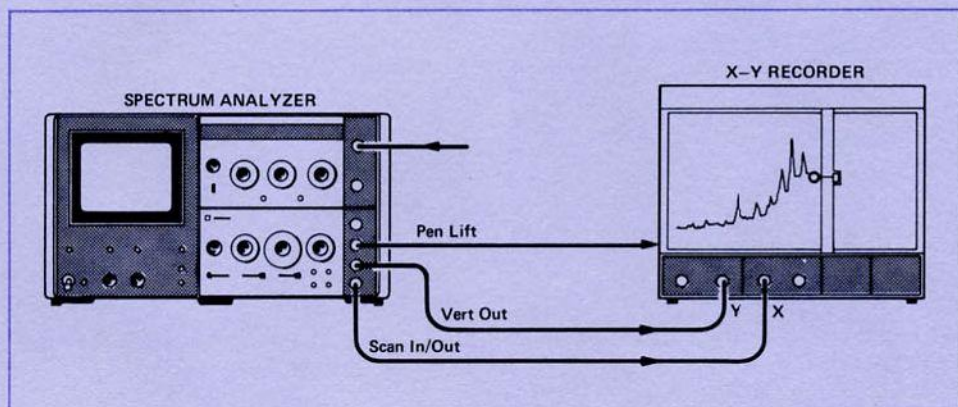
Figure 13. X-Y Recording.
