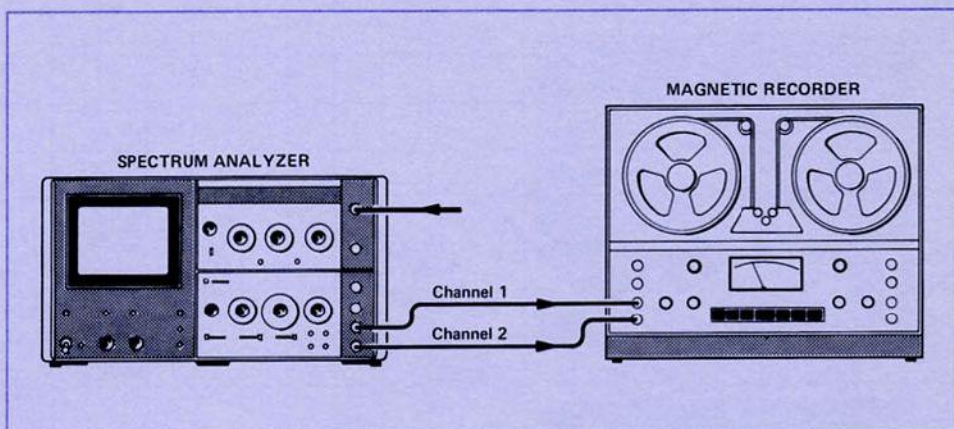
Figure 19. Magnetic Recording.
